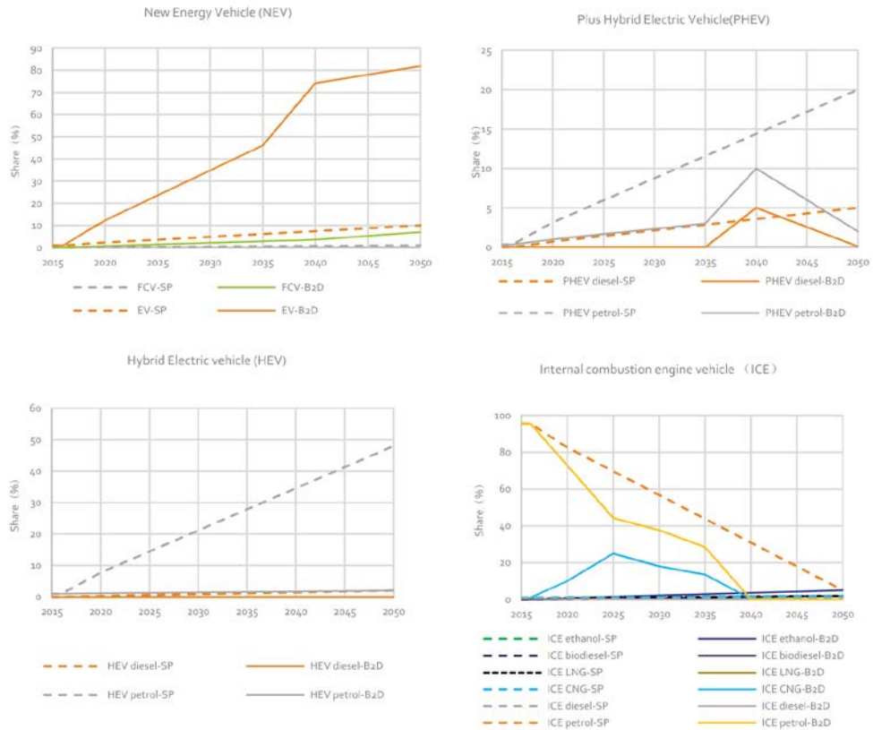
Figure 10-11 Technology proportion in annual sales of passenger vehicles
