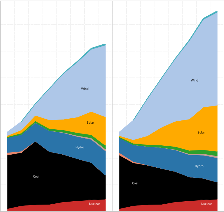
Figure 11-1 Power generation (TWh) from 2016 to 2050 in the two scenarios).
