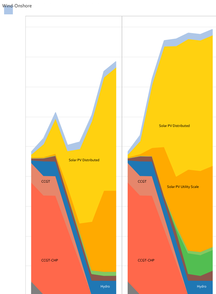
Figure 22-15 Installed Capacity in Beijing (GW) (by power generation type)
