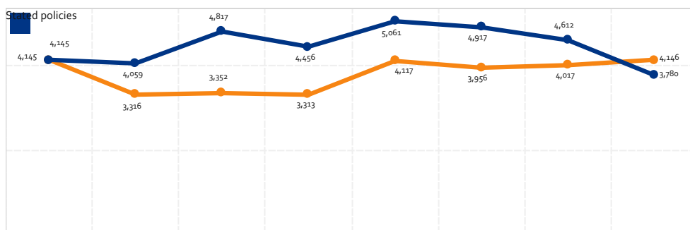
Figure 14-8 Coal power full load hours development in the two scenarios.
