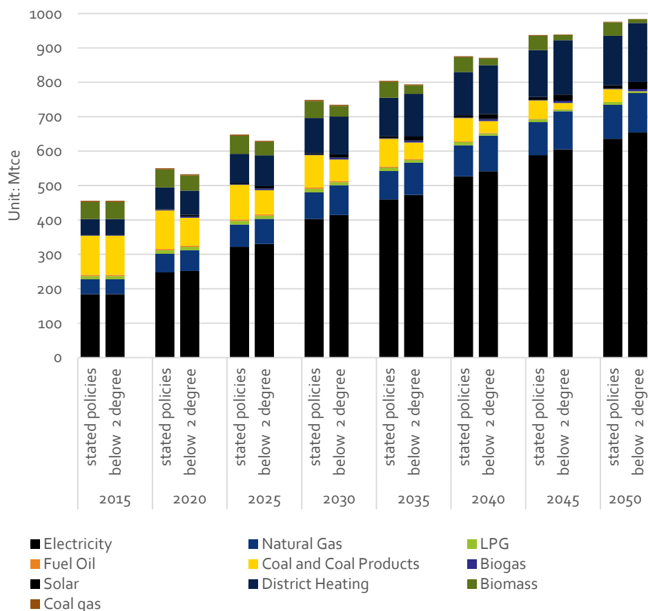
Figure 10-17 Buildings sector's final energy consumption structure
