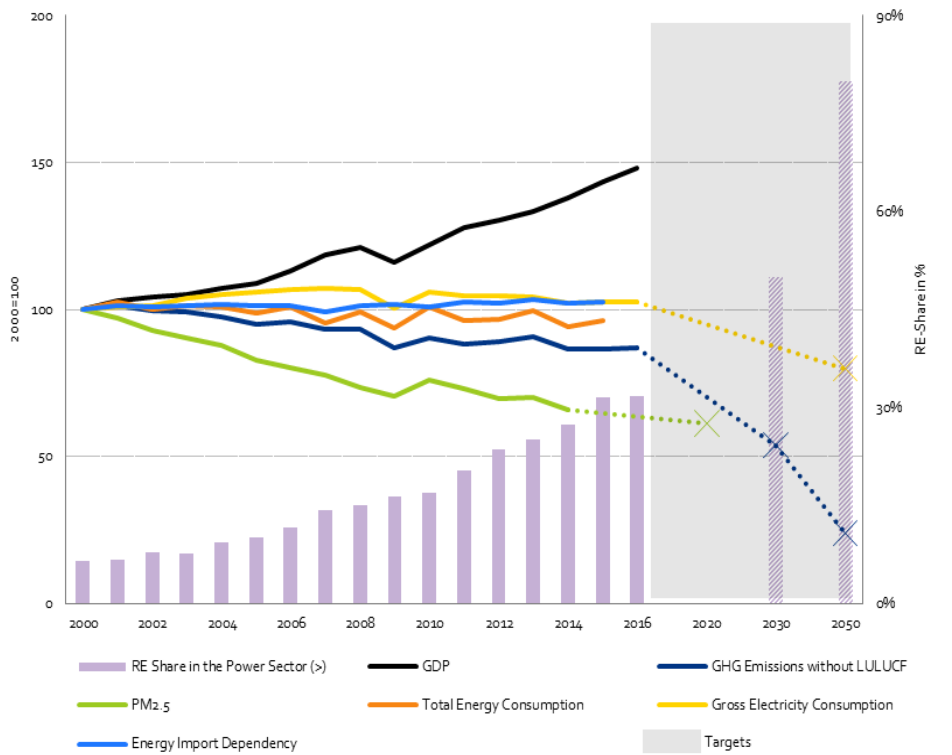
Figure2-4 Key performance indicators for the energy system transition in Germany
