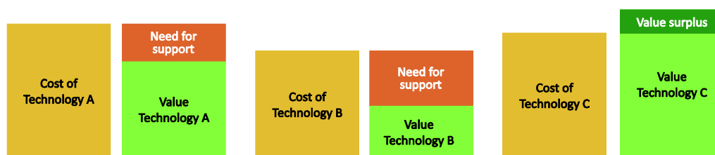
Figure 17-13 The link between VRE cost, SV and competitiveness
