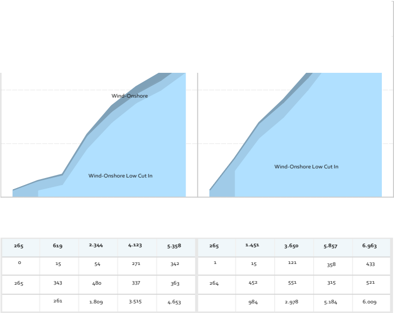
Figure 13-7 Development status of wind power production under different scenarios (TWh)
