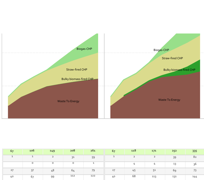
Figure 13-30 National bioenergy generation development (TWh) for the two scenarios.
