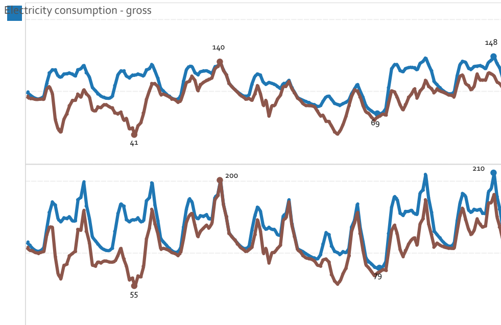
Figure 11-53 Guangdong net-load curve, Electricity consumption minus VRE generation for week 24 in 2050.
