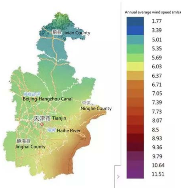
Figure 22-13 Wind Resource Map of Tianjin
