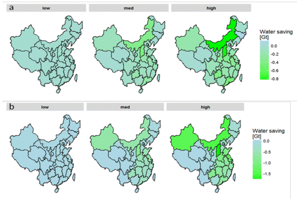
Figure 9-28 Water savings in the Below 2 °C scenario compared with Stated Policies scenario for different water intensities in 2030 (top) and 2050 (bottom)
