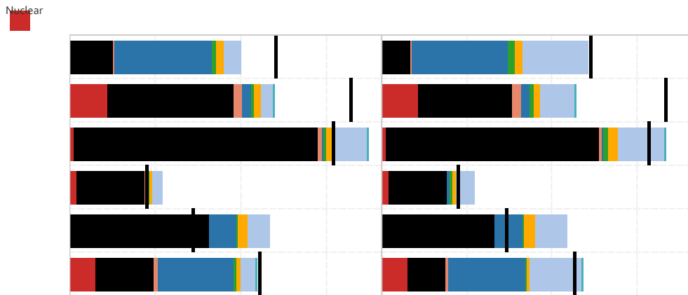
Figure 11-4 Power generation and consumption by regional grid in 2020 (TWh) *
