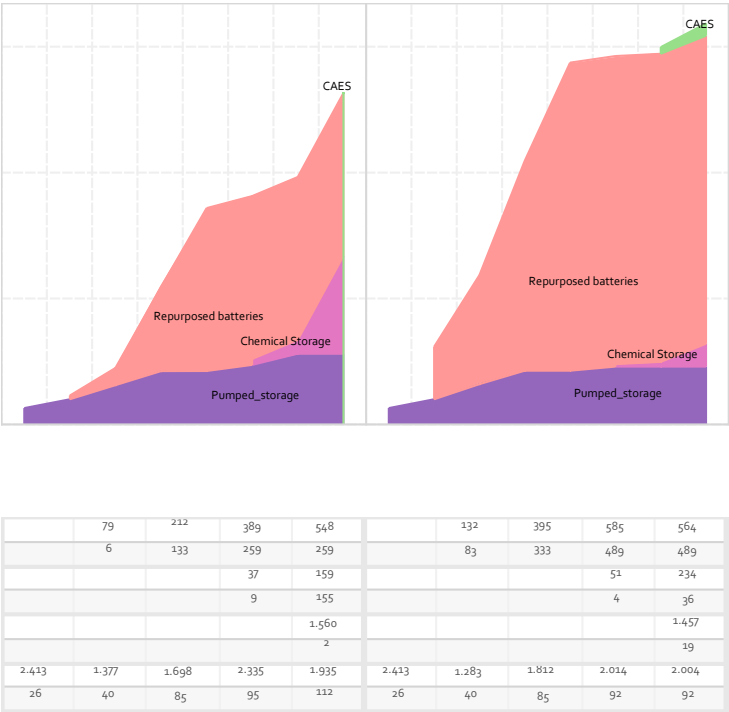
Figure 11-27 Storage capacity (GW) and full load hour development in the two scenarios.
