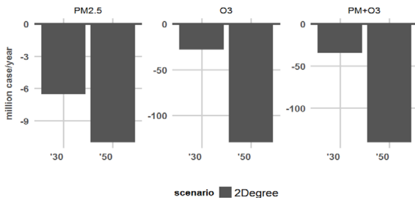
Figure 9-19 Avoided morbidity in the Below 2 °C scenario
