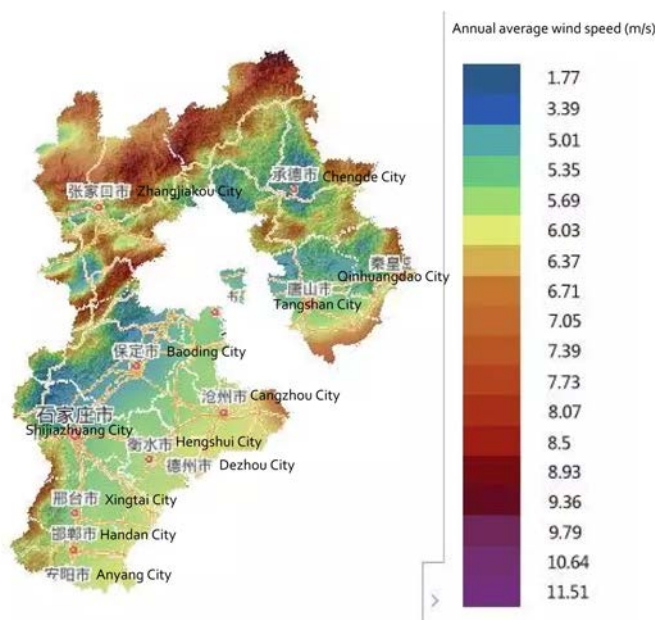
Figure 22-14 Wind Resource Map of Hebei
