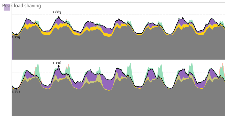
Figure 11-37 National power consumption during week 11 in 2050 in the two scenarios (GW).
