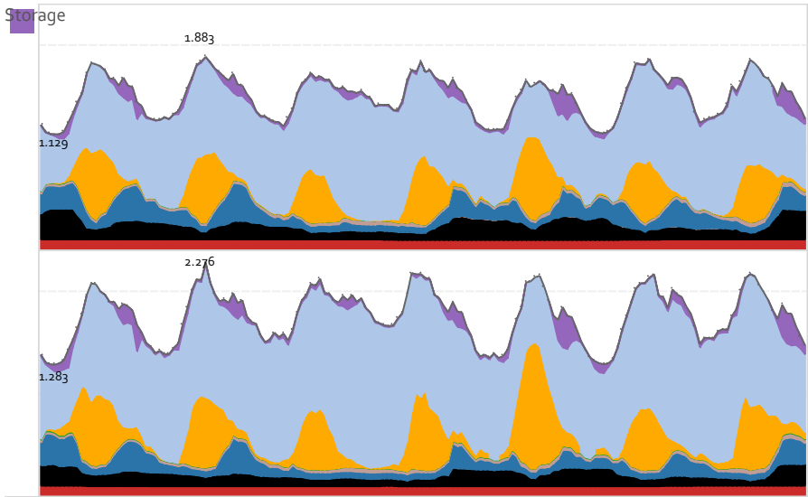
Figure 11-38 Power generation during week 11 in 2050 in the two scenarios (GW).
