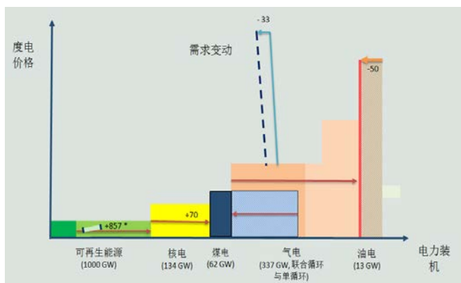
Figure 17-2 Merit-order curve illustration
