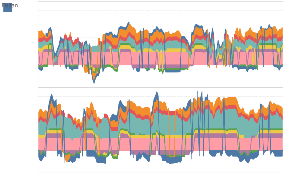
Figure 11-51 Guangdong interprovincial net-imports week 24 in 2050 (GW).
