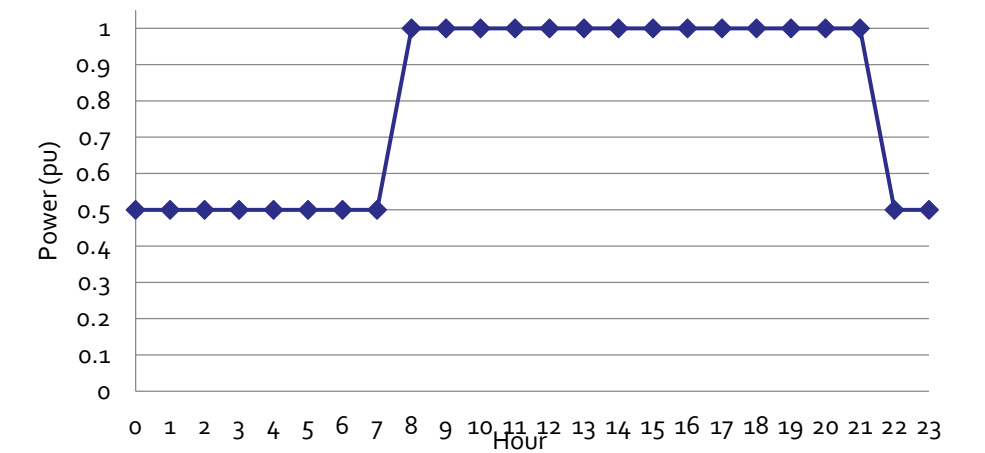
Figure 18-25 Typical power curve of the Chinese HVDC link
