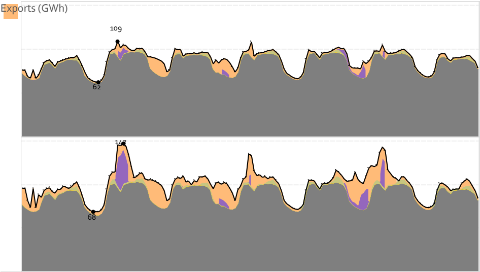
Figure 11-43 Guangdong consumption and exports week 50 in 2030 (GW).
