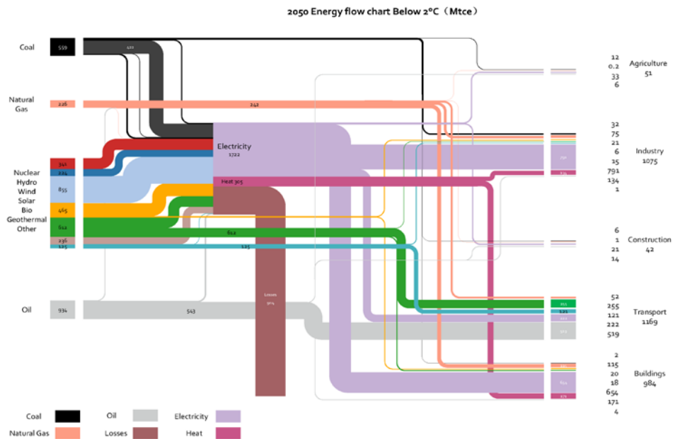
Figure 9-3 Energy flow chart for the Chinese energy system in 2050 for the Below 2 °C scenario
