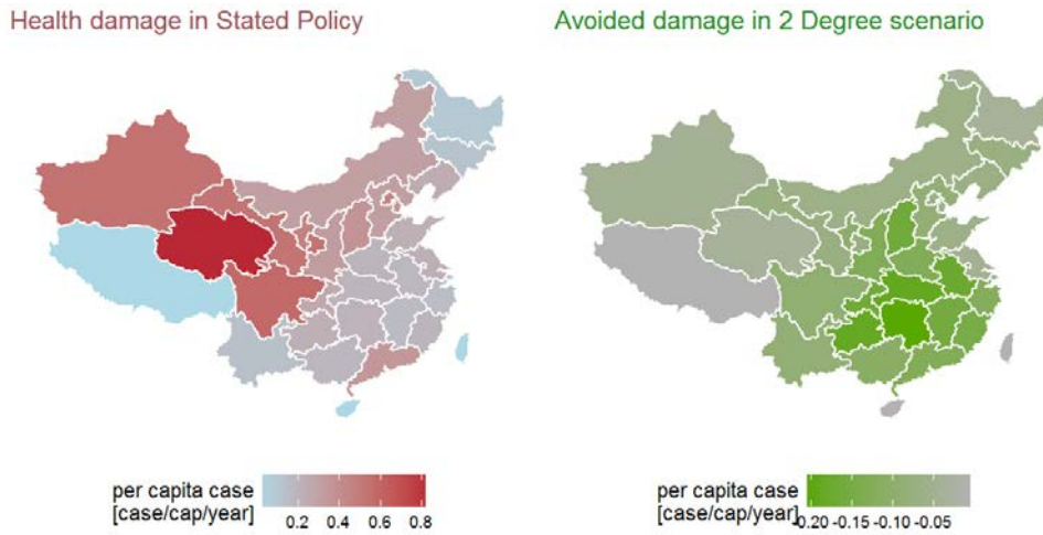
Figure 9-21 Health impacts and benefit on risk of morbidity from PM 2.5 and O 3 in 2050
