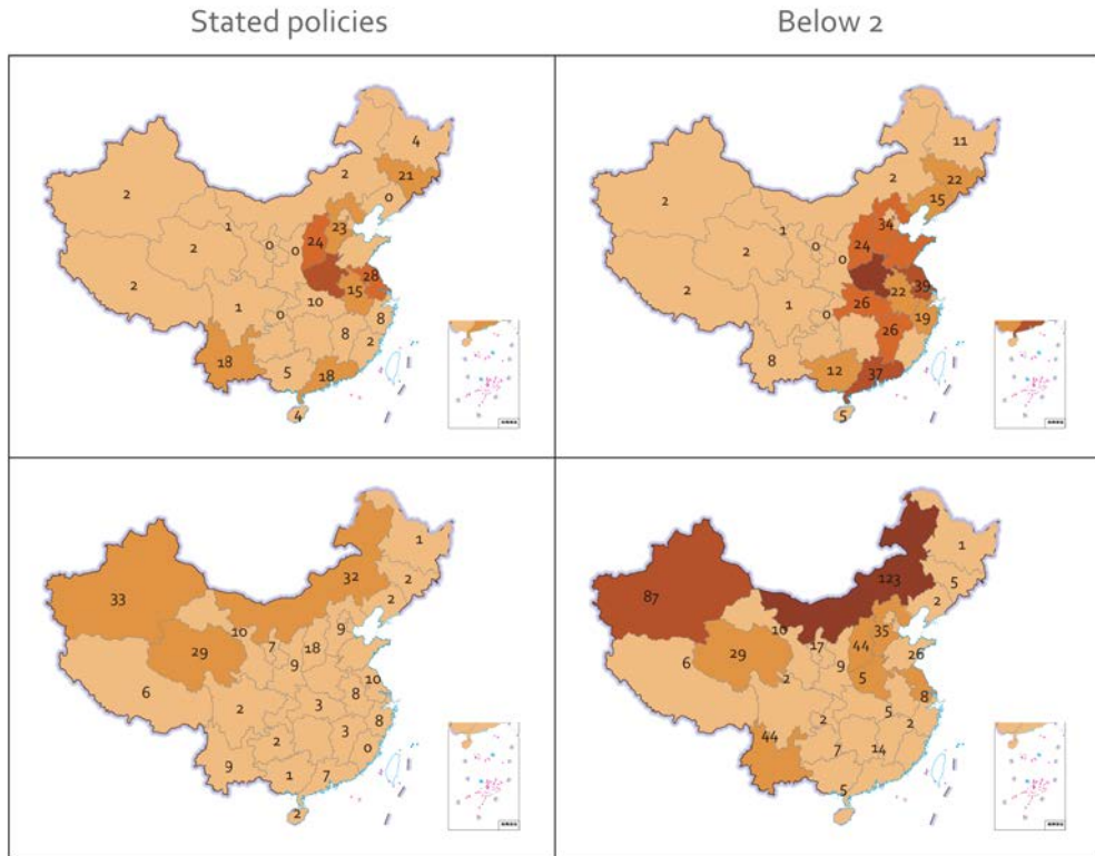
Figure 12-23 Distributed (top) and utility scale (bottom) solar PV installation capacity of by province in the Stated Policies scenario (left) and Below 2 °C scenario (right) in 2030.
