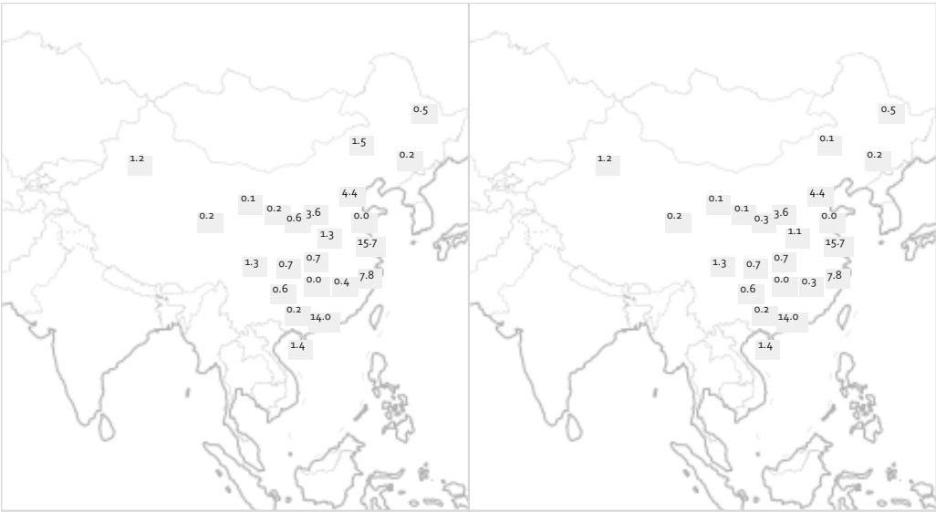
Figure 14-17 Installed natural gas capacity (GW) by province in 2020.
