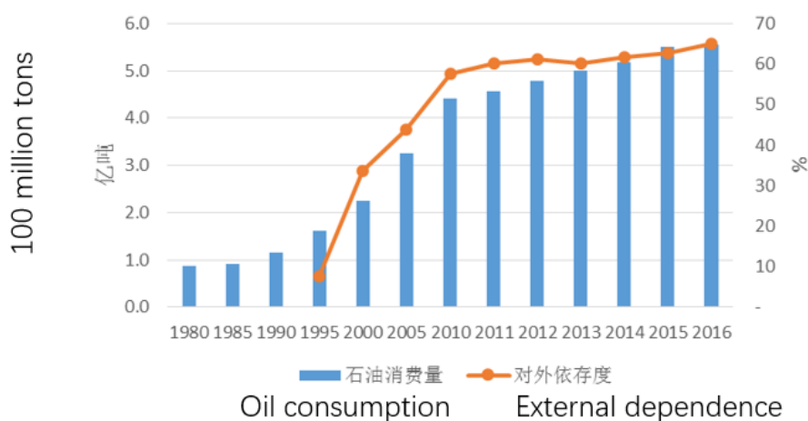
Figure 4-6 Oil consumption and degree of external dependence
