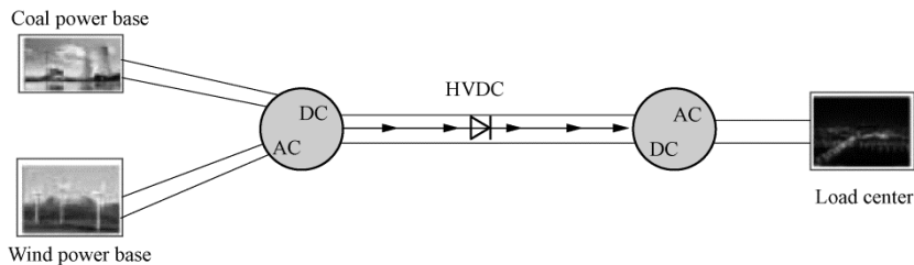
Figure 18-26 Traditional HVDC Scheme with Wind Power Combined with Thermal Power [7]
