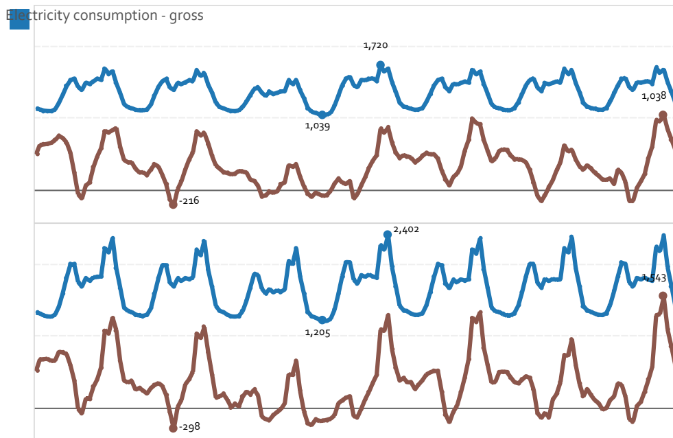
Figure 11-39 Net-load curve, Electricity consumption minus VRE generation for week 11 in 2050.
