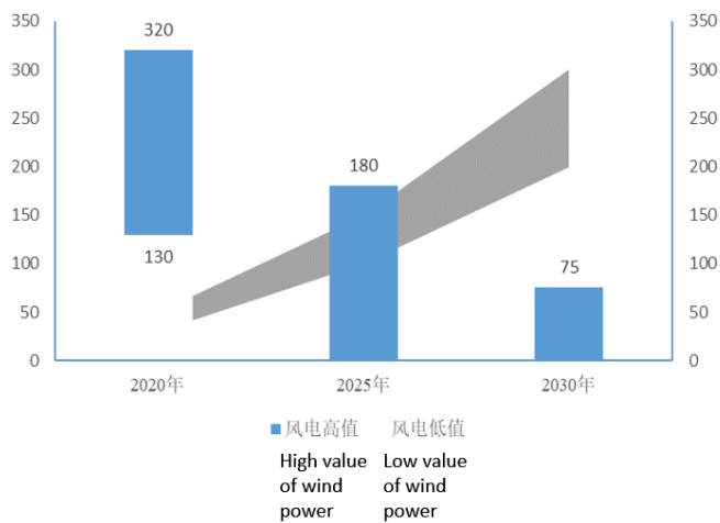
Figure 21-14 Carbon prices of new wind and coal-fired power plants at the same LCOE
