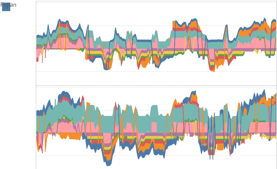
Figure 11-52 Guangdong interprovincial net-imports week 50 in 2050 (GW).
