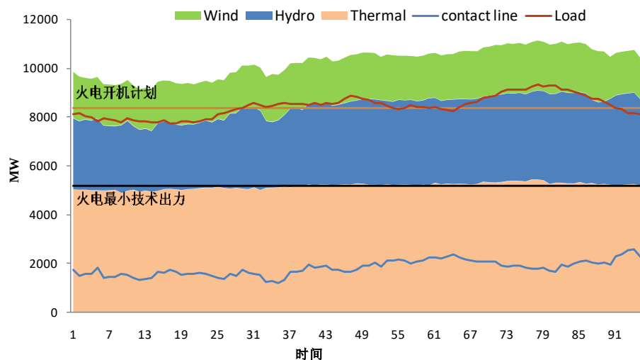
Figure 17-3 Baseload coal power during system operation in Gansu, China
