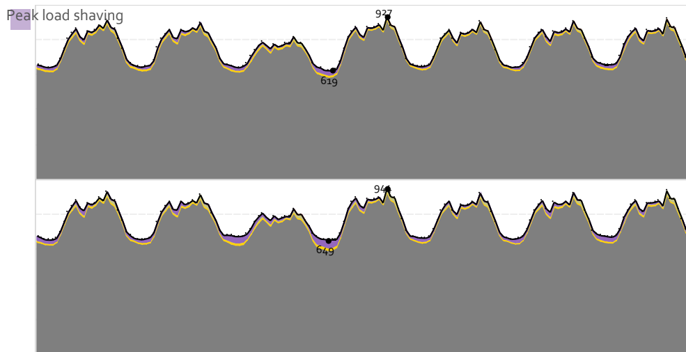
Figure 11-32 National power consumption during week 11 in 2020 in the two scenarios (GW).
