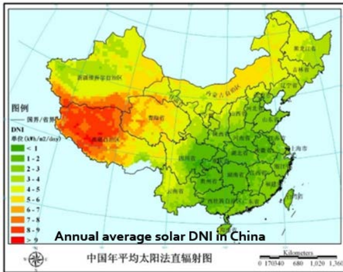
Figure 13-16 annual average solar DNI in China
