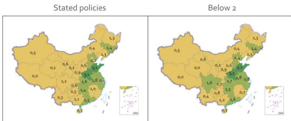
Figure 13-32 Installed bioenergy power capacity (GW) in 2050 in the two scenarios.
