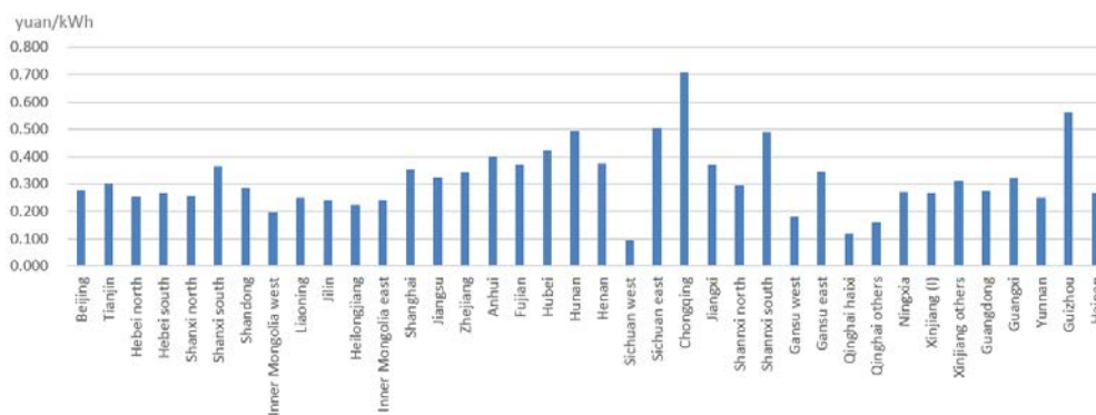
Figure 16-12 Calculation results of FIP demands for large PV plants by region in 2018
