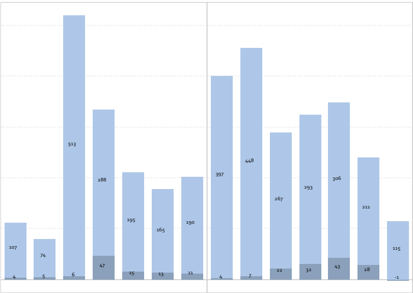
Figure 13-8 Additional capacity in the two scenarios (GW)
