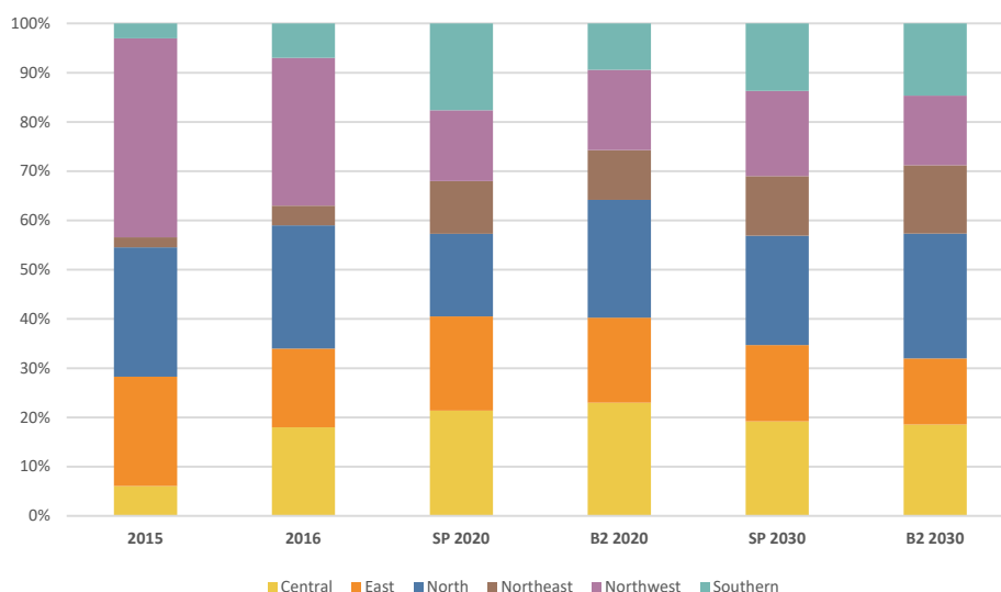
Figure 13-24 Market distribution of solar PV power generation in 2015, 2016 and for the Stated Policies scenario (SP) and Below 2 °C scenario (B2) for 2020 and 2030.
