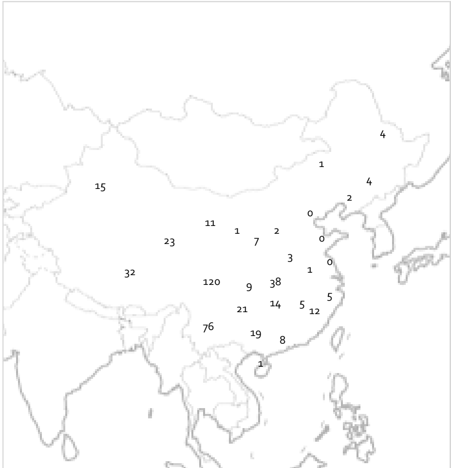
Figure 13-34 China’s hydropower development distribution in 2030 (GW)
