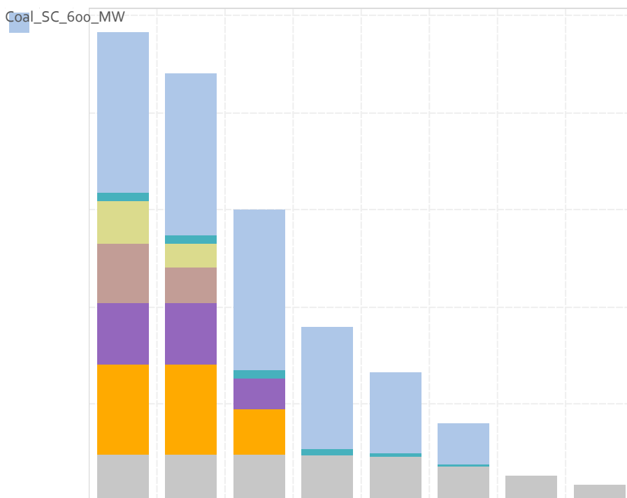
Figure 14-3 Phase out of existing coal capacity without reinvestments
