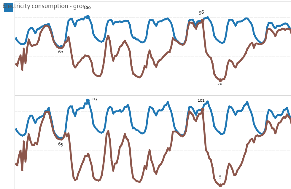
Figure 11-46 Net-load curve, Electricity consumption minus VRE for Guangdong, week 50 in 2050.
