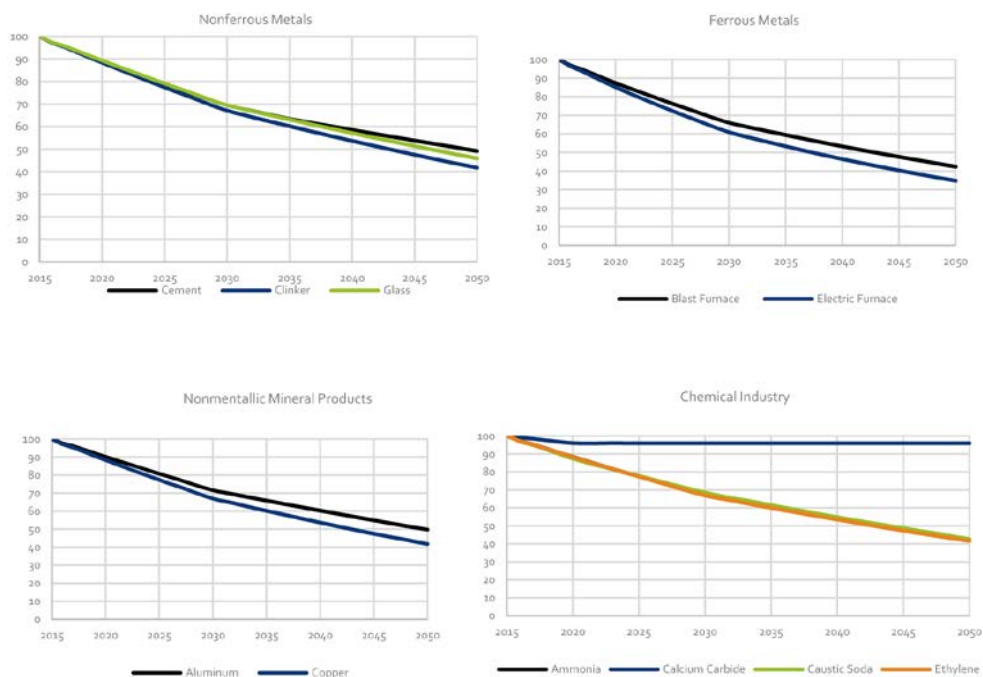
Figure 10-6 Forecasts on energy intensity change of class I Industry during 2015-2050
