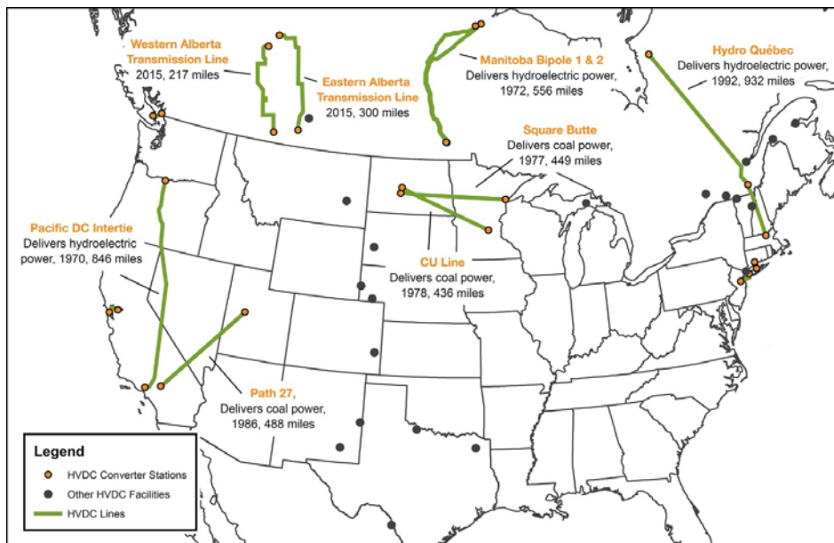
Figure 18-16 HVDC Deployment in North America.
