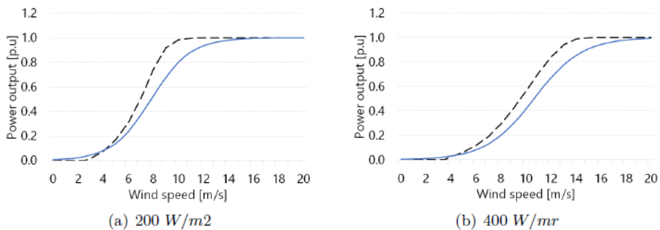
Figure 13-5 Result of power curve smoothing at different wind speeds (blue solid line denotes result of smoothing)
