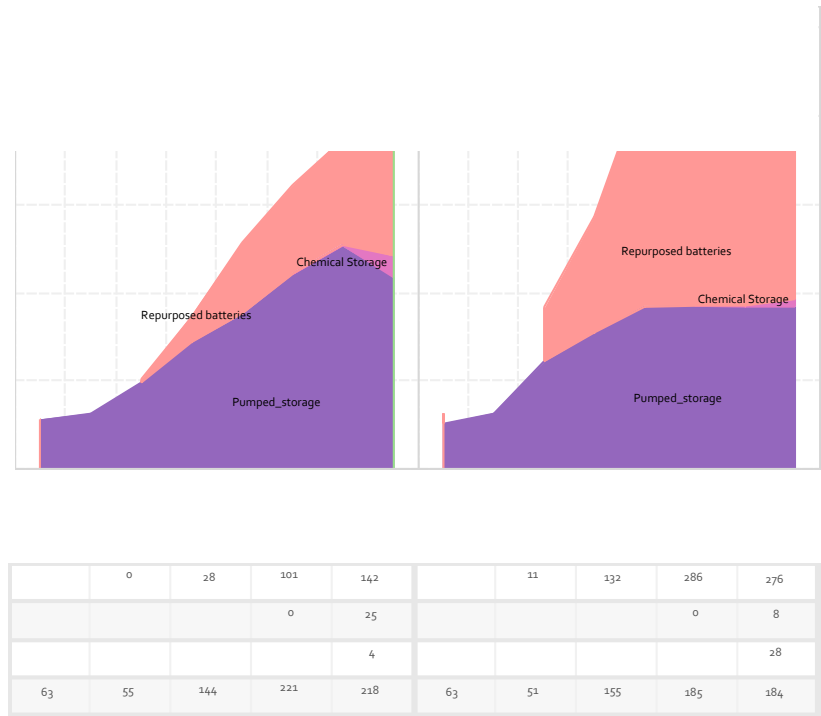
Figure 11-28 Storage capacity (TWh) and full load hour development in the two scenarios.
