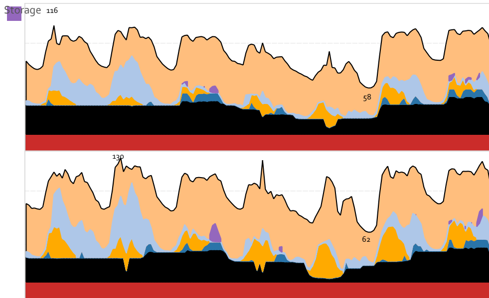
Figure 11-41 Guangdong generation and import (light orange) week 24 in 2030 (GW).
