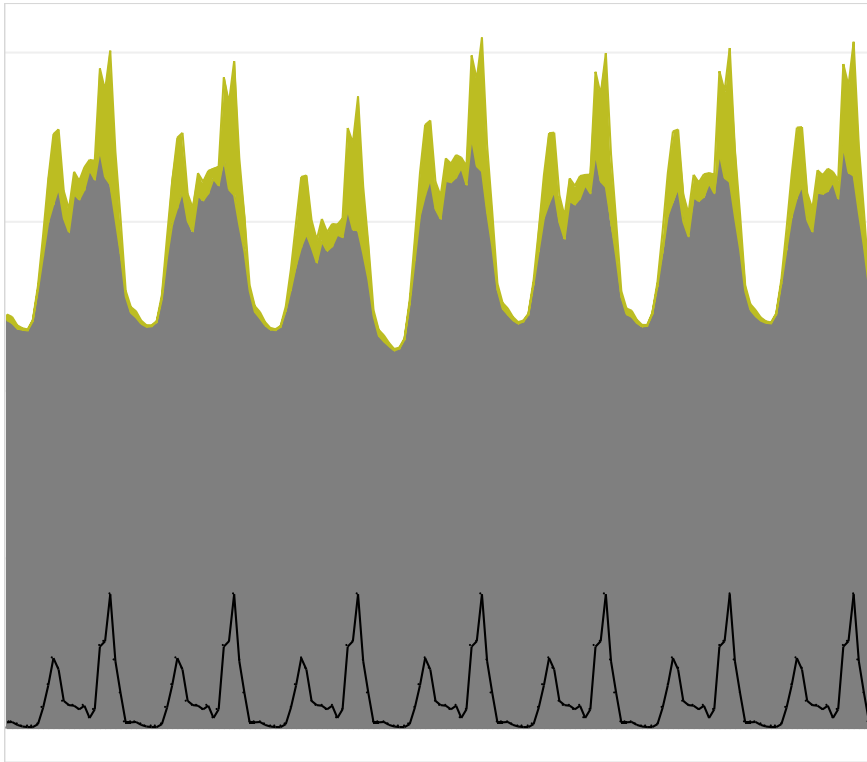
Figure 11-11 Illustration of the exogenous hourly load shape assuming non-smart EV loading (top area and line) and other load in 2050 of the Below 2 °C scenario.
