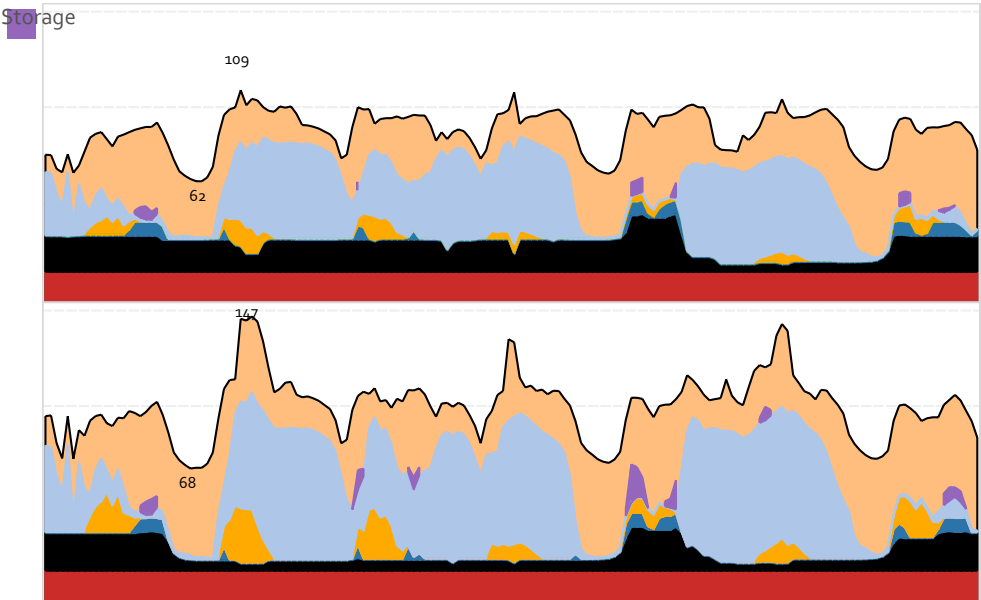
Figure 11-44 Guangdong supply and import week 50 in 2030 in the two scenarios (GW).
