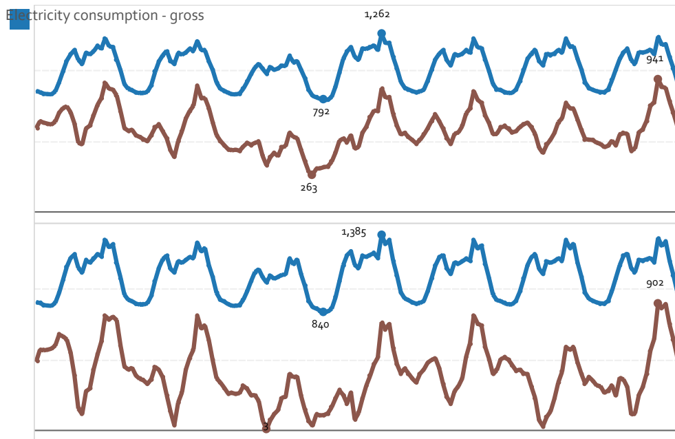
Figure 11-36 Net-load curve, Electricity consumption minus VRE generation for week 11 in 2030.
