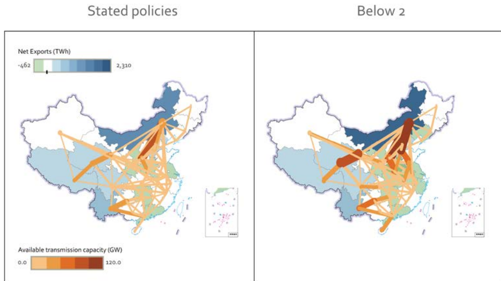
Figure 11-16 Interprovincial transmission capacity and annual net-exports by province in 2050.
