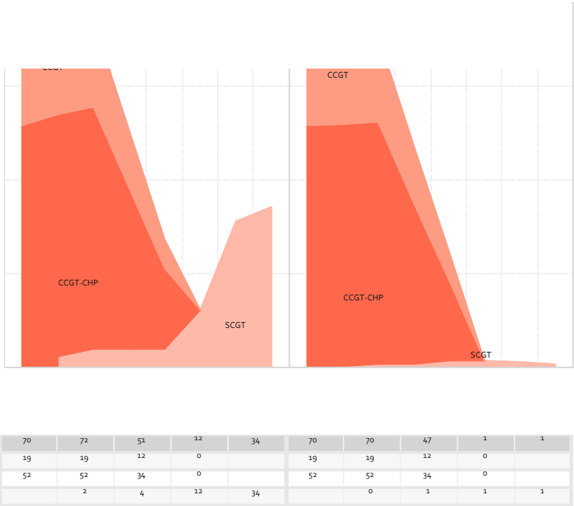
Figure 14-15 Natural gas capacity (GW) development in the two scenarios.
