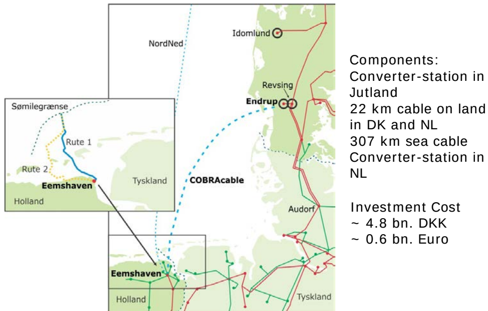
Figure 18-22 The Cobra DC interconnector between Denmark and the Netherlands.
