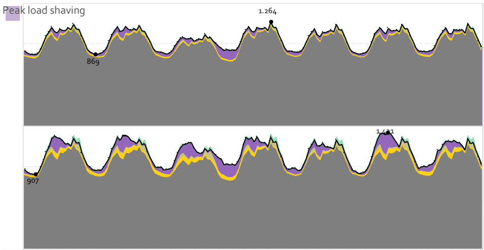
Figure 11-34 National power consumption during week 11 in 2030 in the two scenarios (GW).
