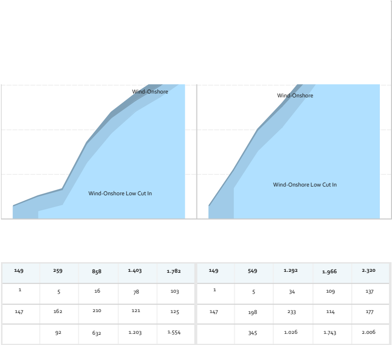
Figure 13-6 Comparison of development status of installed wind power capacity under different scenarios (GW)
