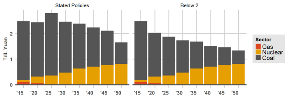
Figure 12-6 Direct output of non-RE power in 2050 (2010 price)
