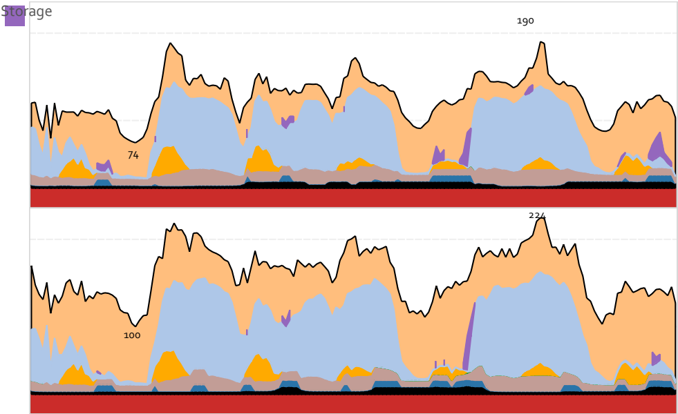
Figure 11-50 Generation and import in Guangdong week 50 in 2050 (GW).
