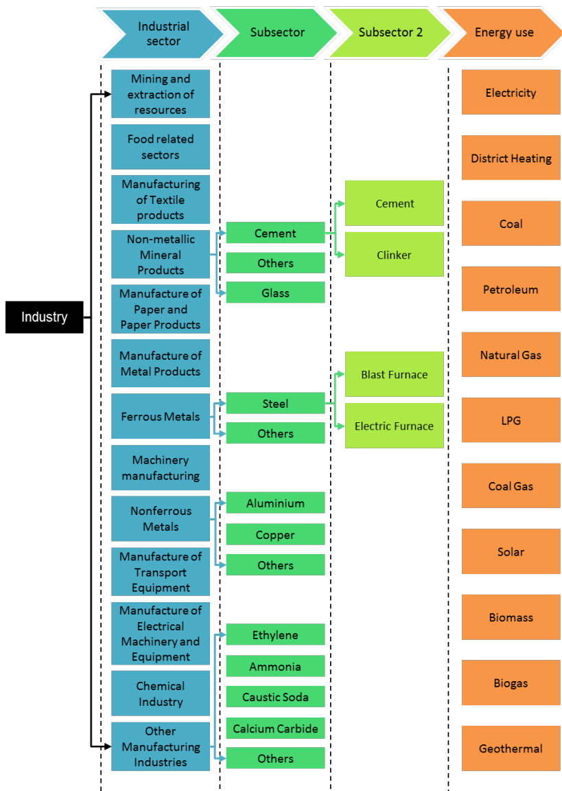
Figure 10-2 industrial sector's final energy demand model framework
