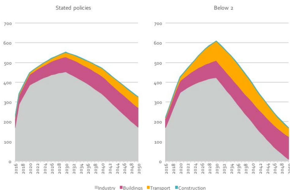
Figure 7: Direct use of natural gas in end-use sectors (Mtce).
