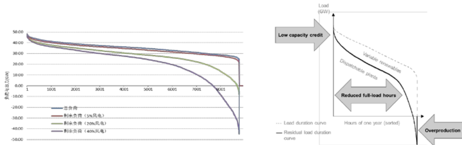
Figure 17-7 Diminishing baseload in residual load curve (Jing-Jin-Tang power grid)
