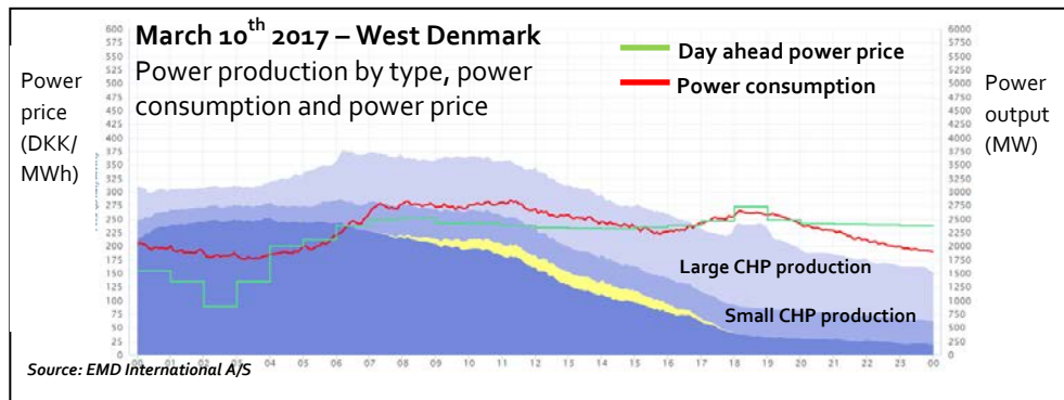
Figure 19-5 One day's power production, consumption and power prices in the Day Ahead market in western Denmark.
